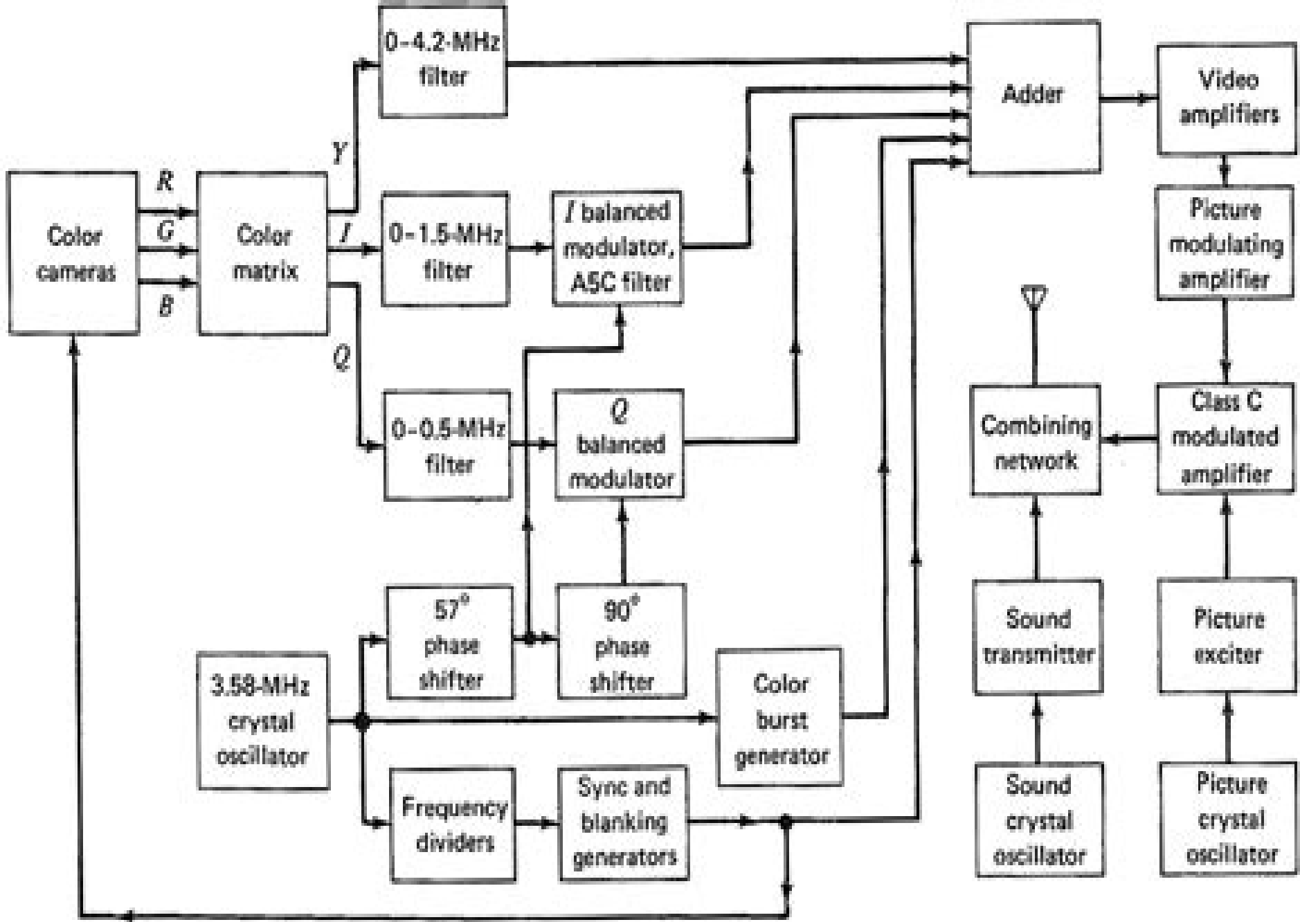
FIGURE 17-22 Basic block diagram of color television transmitter.
