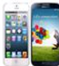
Smart Phones
