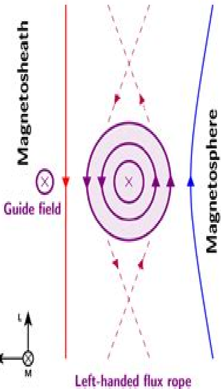
(a) View from the Dusk
