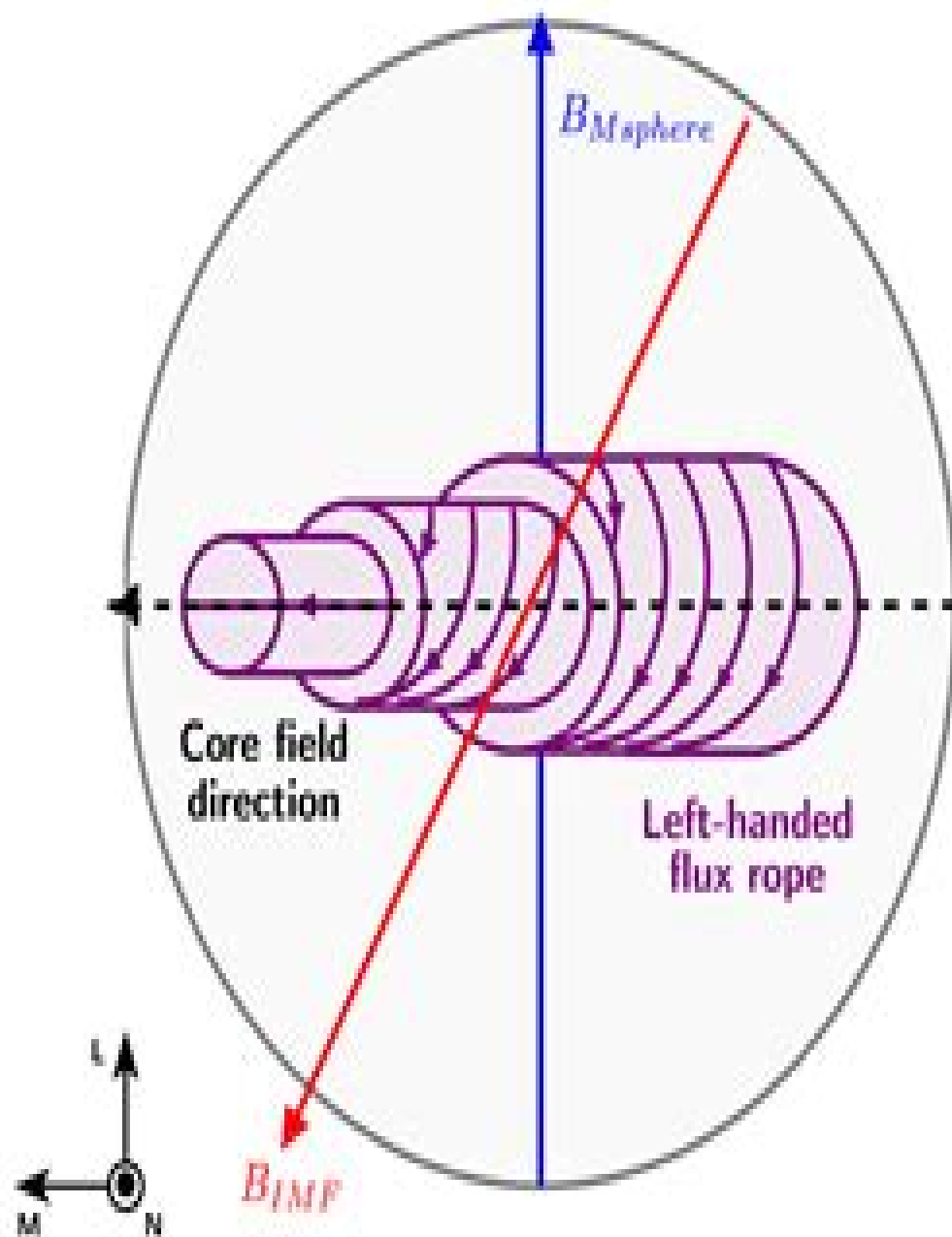
(b) View from the Sun
