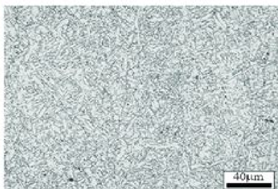
weld D (0.5Mn,Al / O=0.81)
