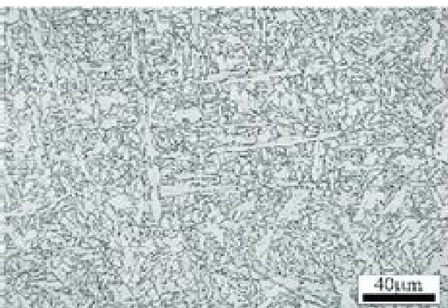
weld C (0.5Mn,Al / O=0.43)
