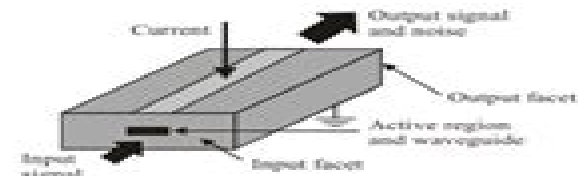
Fig. 1: Schematic diagram of an SOA.
