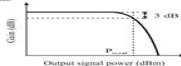
Fig. 3: Typical SOA gain versus output signal power.
