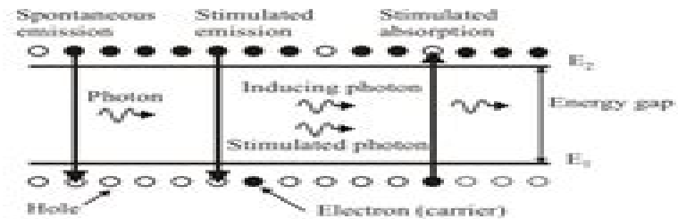
Fig. 2: Spontaneous and stimulated processes in a two level system.
