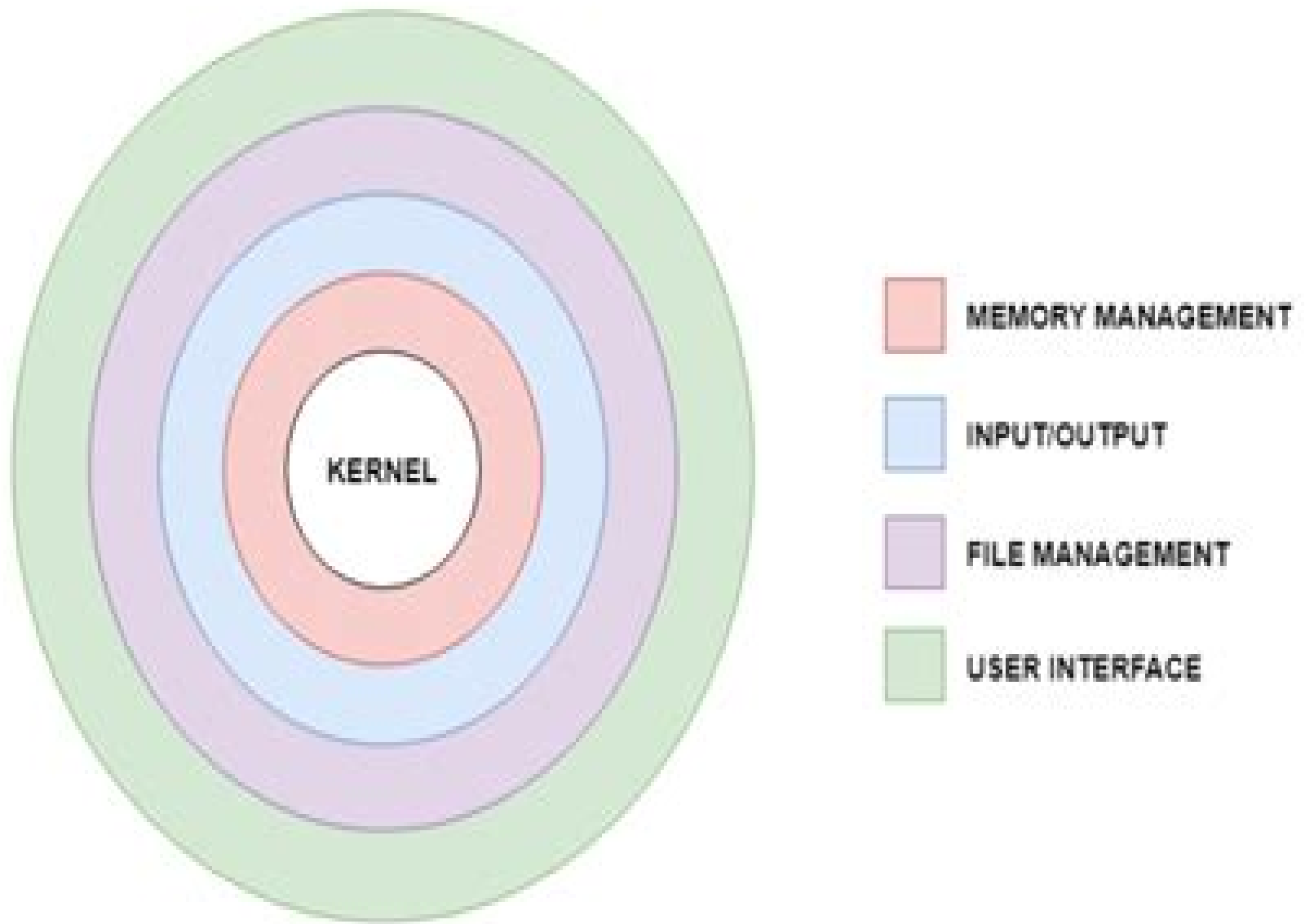
Layered Operating System Design
