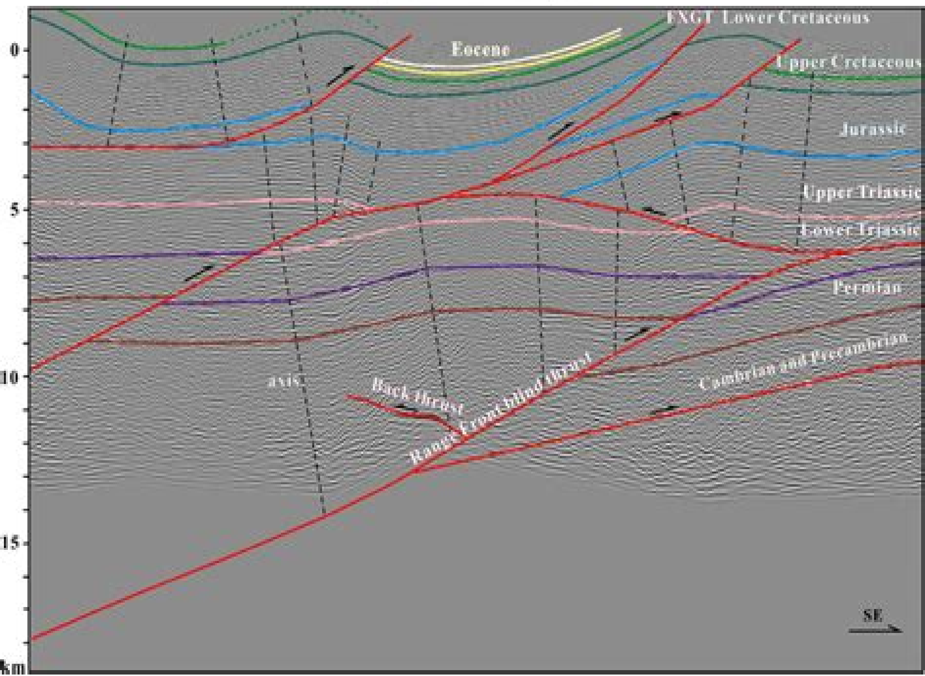
Seismic reflection profile 1
