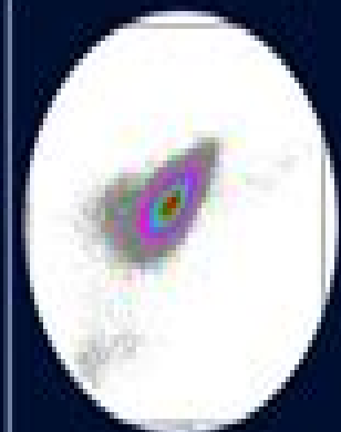
Flow Cytometry
