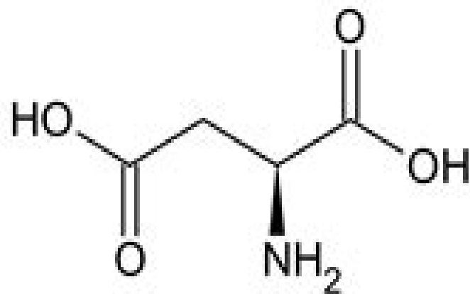
Aspartic acid
