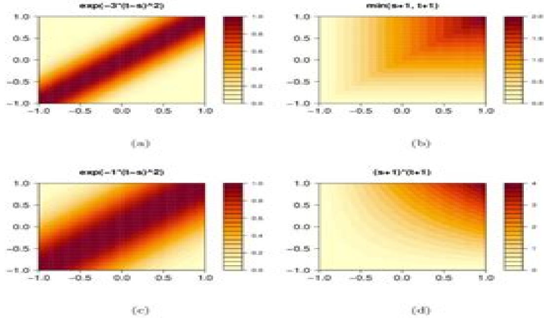
Figure 5: Simulation III: Contour plots of prior covariance functions.
