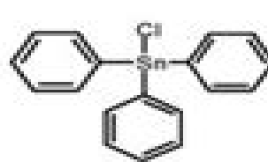
Triphenyltin chloride
