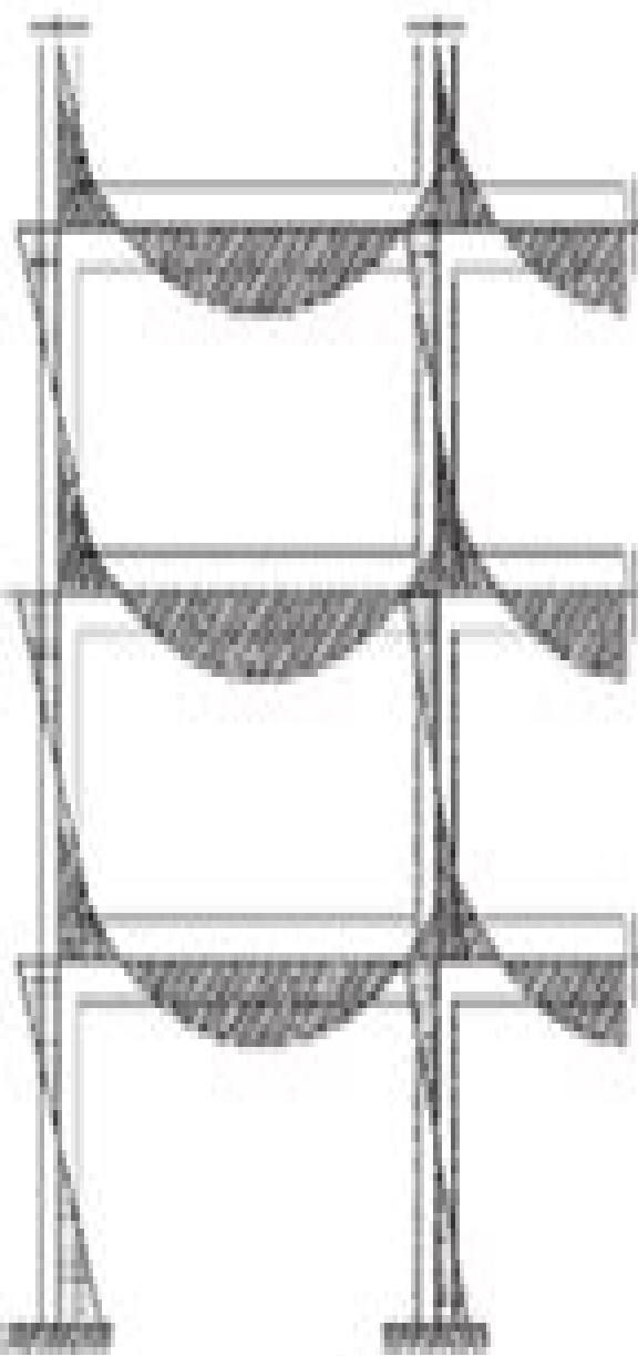
a) Original B.M.D
