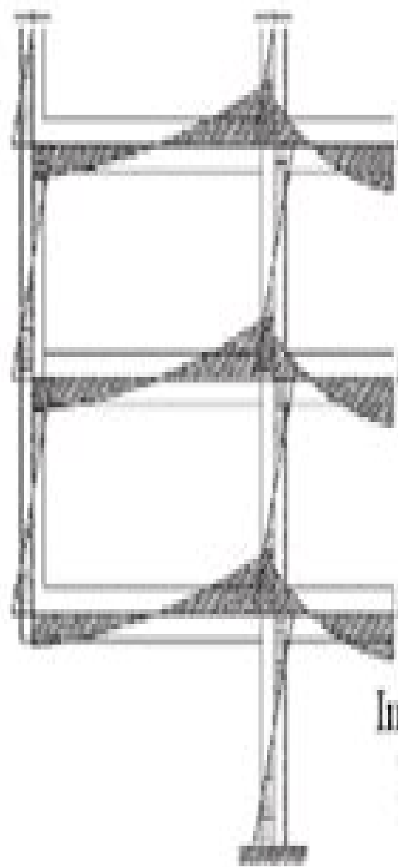
b) B.M.D after column loss
