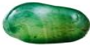
green agate
