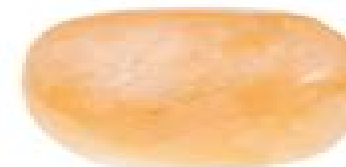
stilbite
