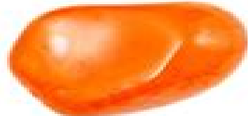
carnelian (chalcedony)
