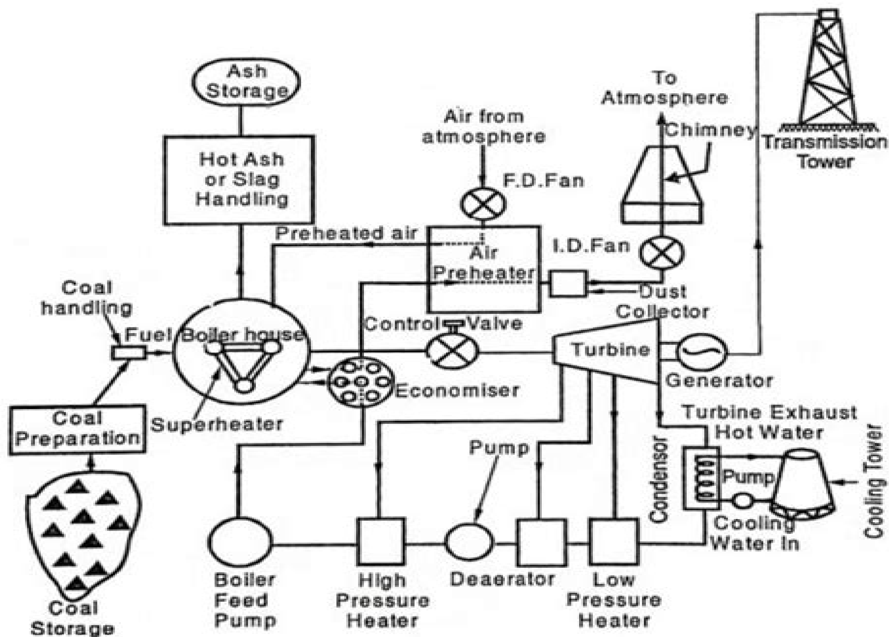
Fig: 1.26 Steam Power Plant or Thermal Power Plant
