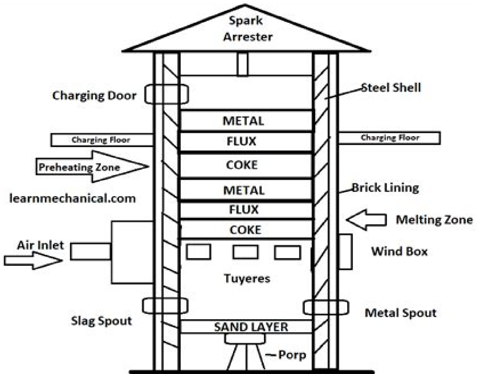
CUPOLA FURNACE
