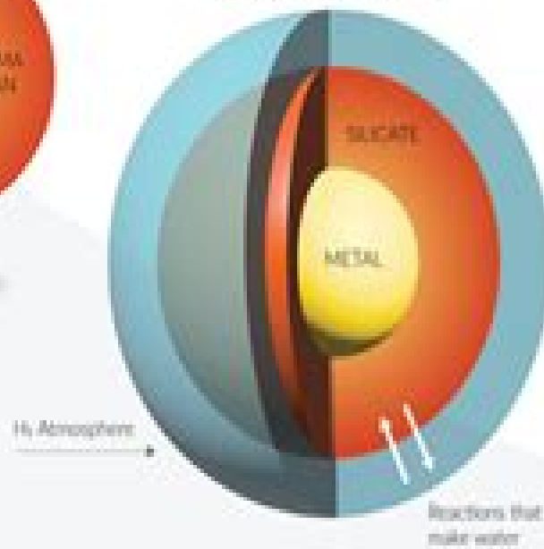
PLANETARY EMBRYO & H_2 ATMOSPHERE
