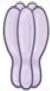
NICOTINIC RECEPTOR
