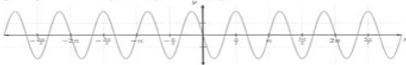
Figure 2.19: Graph y = -2 \sin 3x
