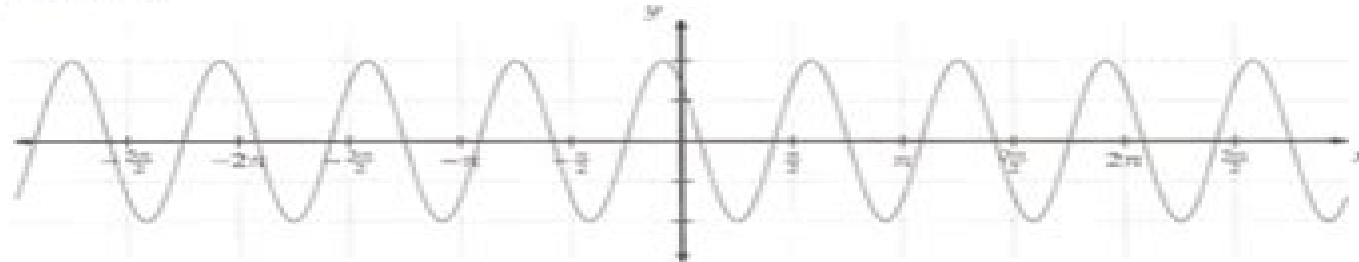
Figure 2.20: Graph y = -2 \sin(3x - \frac{\pi}{4})
