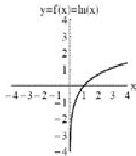
Natural Logarithmic Function
