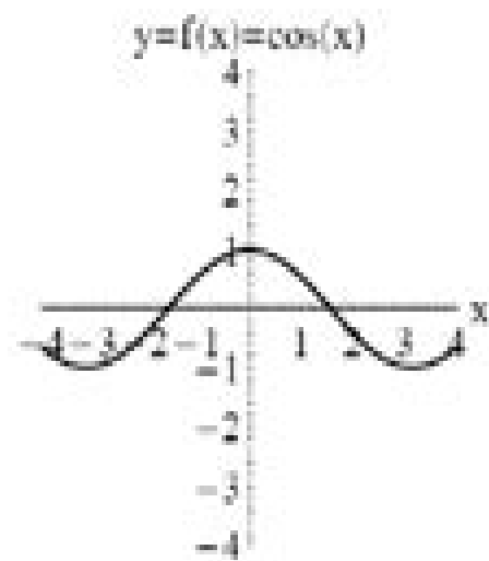
Cosine Function
