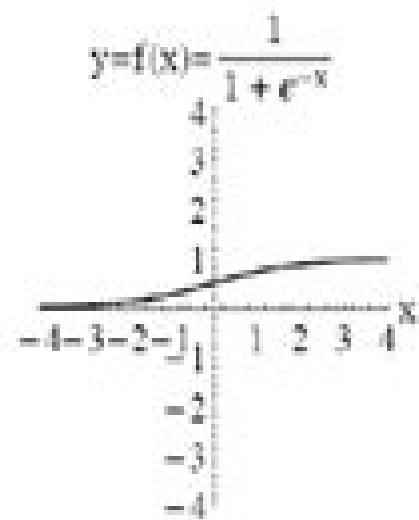
Logistic Function
