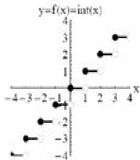
Greatest Integer Function
