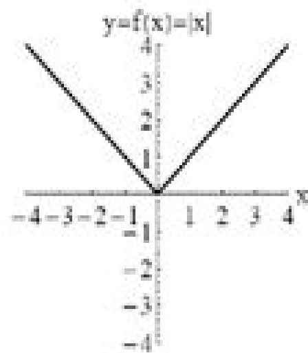
Absolute Value Function
