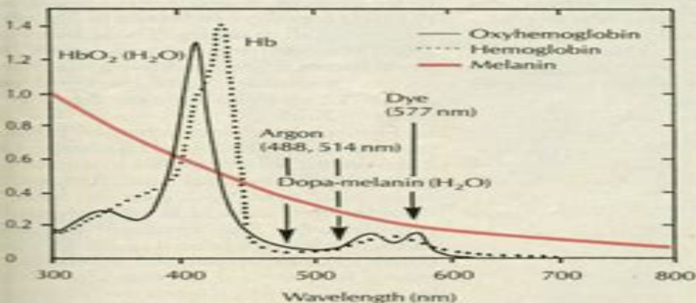
FIGURE 1. Absorption spectrum of oxyhemoglobin, hemoglobin and melanin. emission wavelengths of dye and argon lasers.
