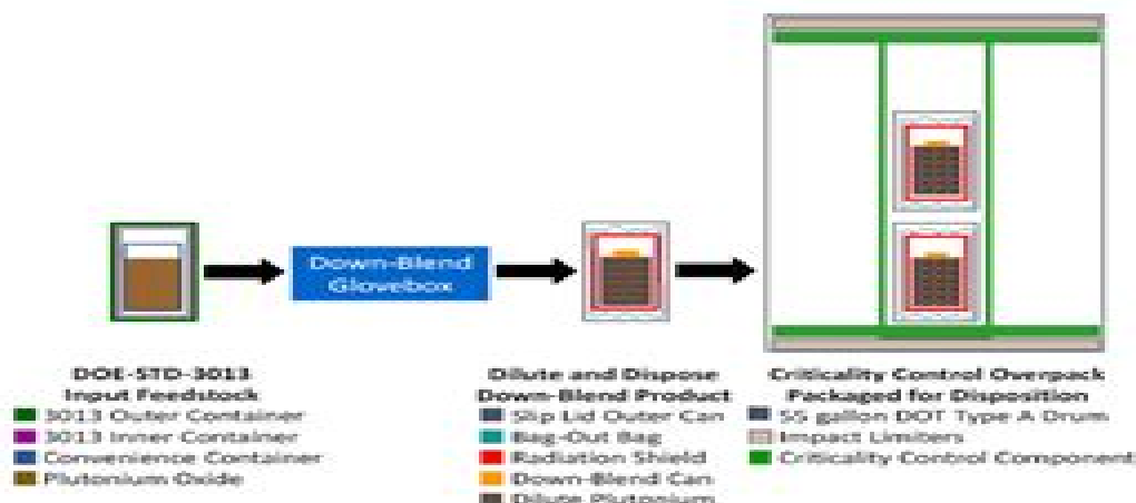
FIGURE 2-3b Cross sections of the plutonium containers used in the process outlined in Figure 2-3a. At Los Alamos National Laboratory, the oxidized plutonium is placed into DOE-STD-3013 containers. Upon arrival at the Savannah River Site, the same containers are used to store the plutonium oxide until it is introduced into the glovebox. The can/bag/can assembly described and shown in Figure 2-3a is shown here as “Dilute and Dispose Down-Blend Product.” Two of these assemblies are placed within a stainless steel pipe, the Criticality Controlled Component (CCC). A single CCC is placed inside a Criticality Controlled Overpack (CCO). The CCO is a 55-gallon drum. SOURCE: Adapted from image provided by the U.S. Department of Energy (McAlhany 2017).
