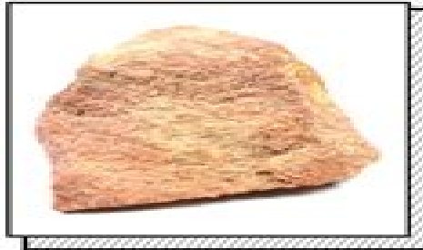
SEDIMENTARY ROCK
