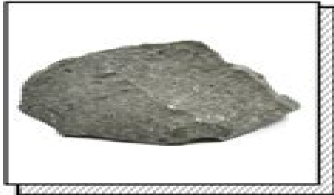
IGNEOUS ROCK
