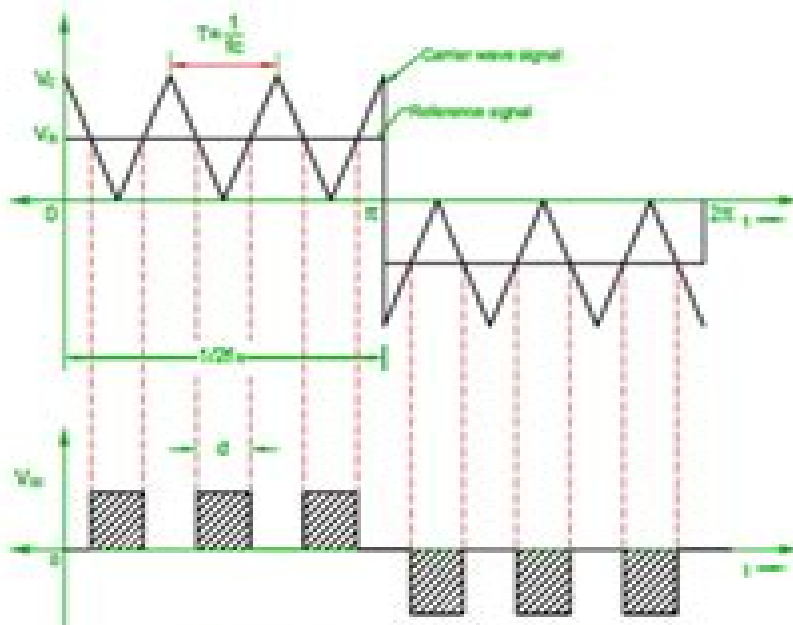
FIG 2: MULTIPLE PULSE WIDTH MODULATION
