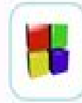
CODE::BLOCKS
