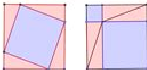
Pythagoras' Theorem: c^2 = a^2 + b^2
