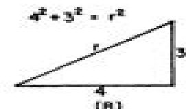
Figure 19-2.—The Pythagorean Theorem.
