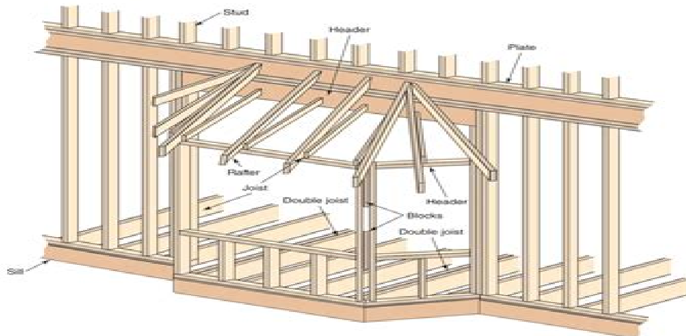
Figure 11-31. Traditional framing for a bay window. To illustrate how joists are extended over the sill, the subfloor is not shown here. Joists at either side of the extension should be doubled.
