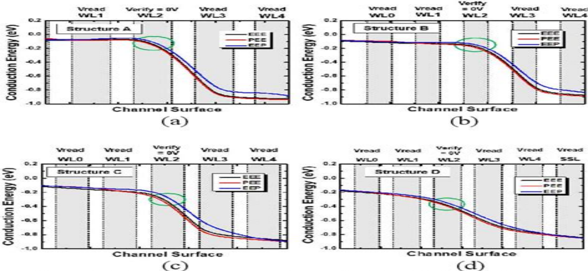
Figure 4. Conduction energy at channel surface during read operation (a) structure A, (b) structure B, (c) structure C, (d) structure D.
