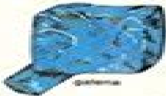
twin crystals
