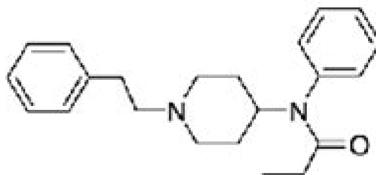
Fentanyl
