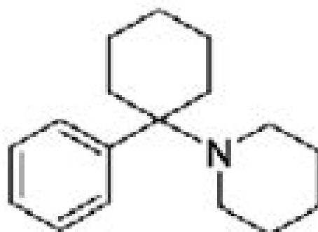
Phencyclidine (SN)
