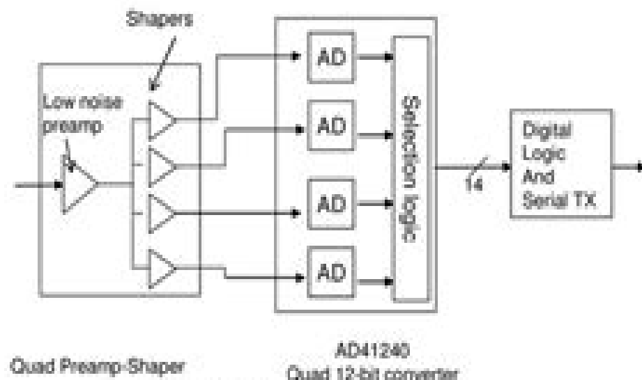
System architecture
