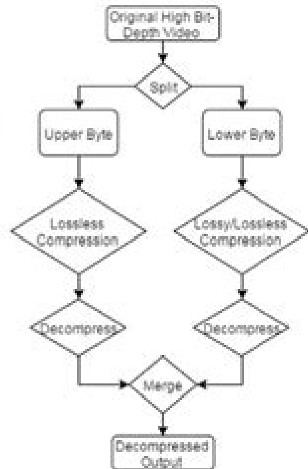
Bit-Stream Splitting
