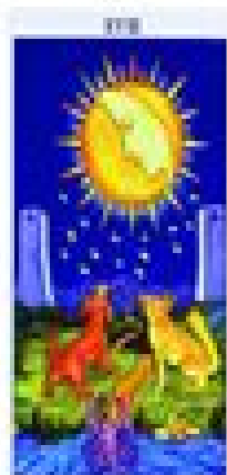
THE MOON
