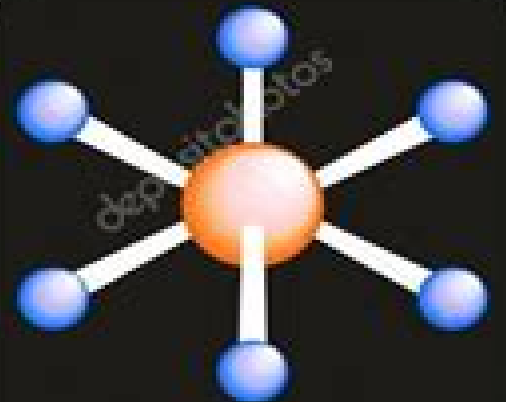
Octahedral
