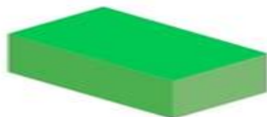
cuboid
