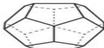
dodecahedron
