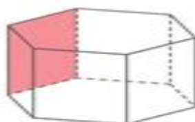
hexagonal prism
