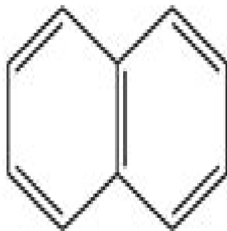
Naphthalene
