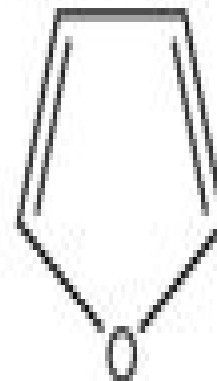
Furan
