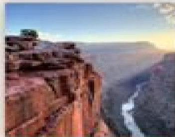
Grand Canyon
