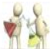
Dimethyl carbonate
