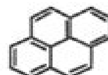
Pyrene 202.3 g
