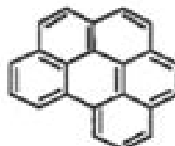
Benzo[g,h,i]perylene 276.3 g
