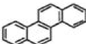
Chrysene 228.3 g
