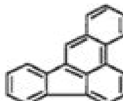
Benzo[b]fluoranthene 252.3 g
