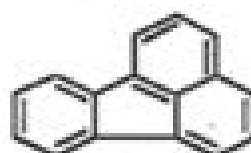
Fluoranthene 202.3 g
