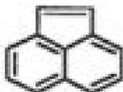
Acenaphthylene 152.2 g
