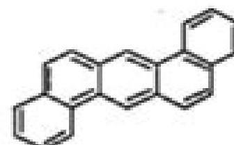
Dibenz[a,h]anthracene 278.4 g
