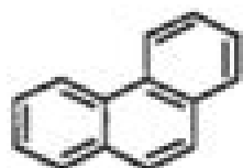
Phenanthrene 178.2 g
