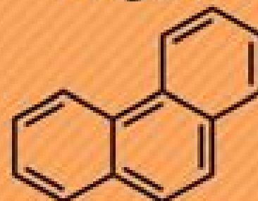
Phenanthrene
