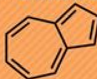
Azulene
