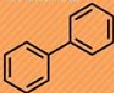
Biphenyl
