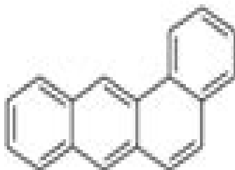
Benz[a]anthracene
