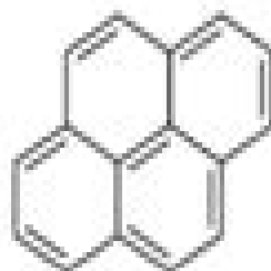
Pyrene
