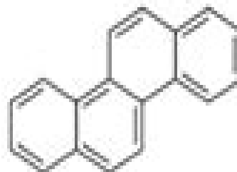
Chrysene
