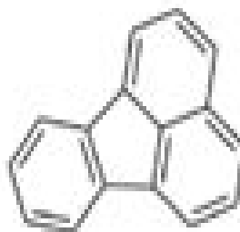
Fluoranthene
