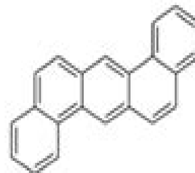
Dibenz[a,h]anthracene
