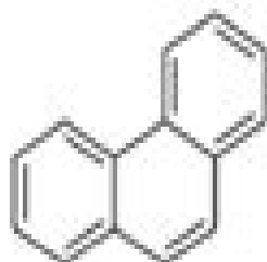
Phenanthrene
