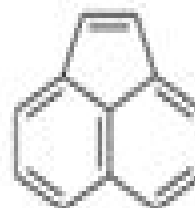
Acenaphthylene
