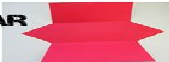
OCTAHEDRON
