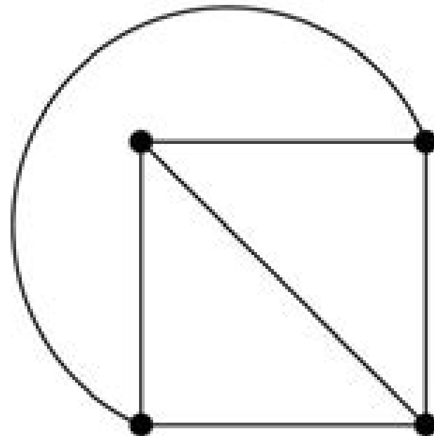
FIGURE 2 The Graph K_4 . FIGURE 3 K_4 Drawn with No Crossings.
