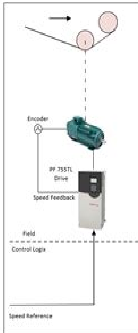
Speed control
