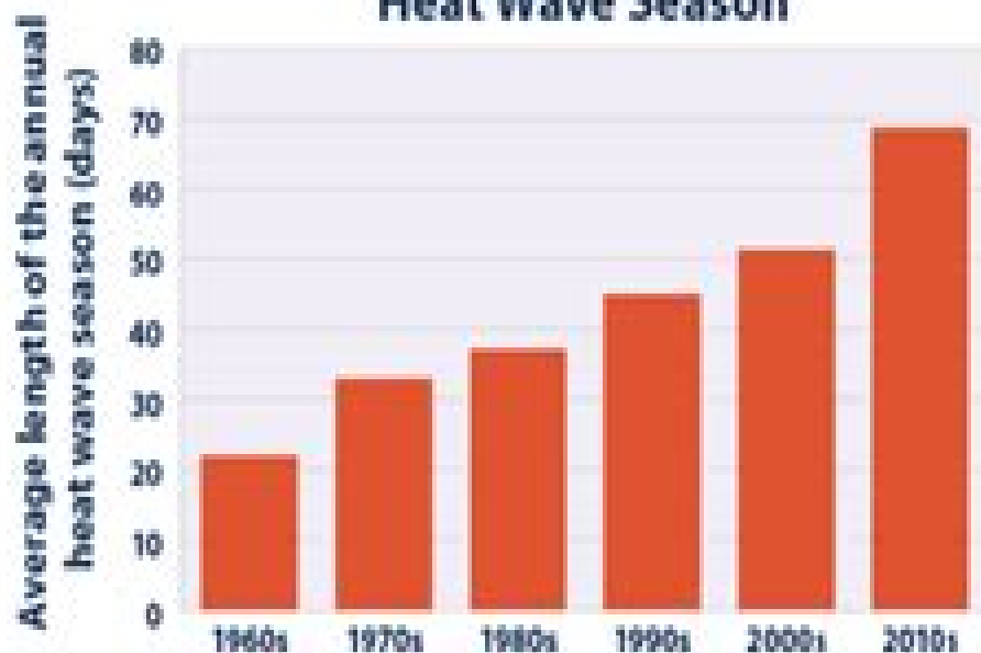
Heat Wave Season
