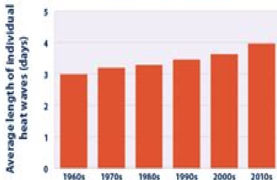
Heat Wave Duration
