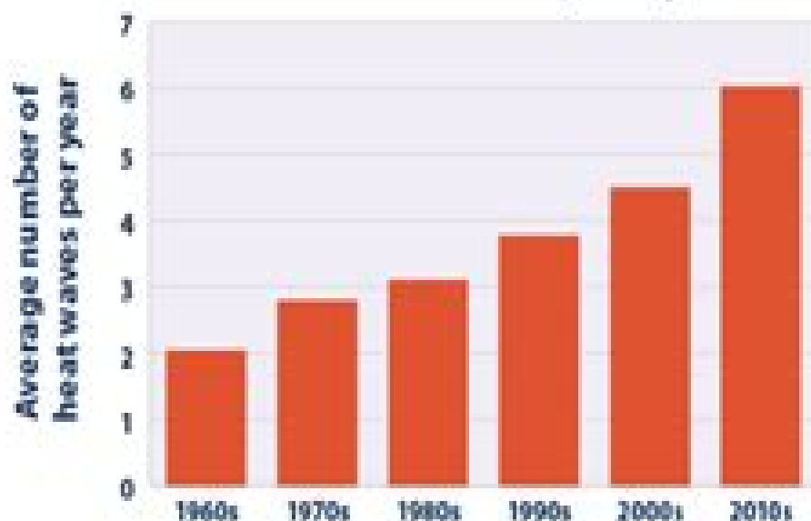
Heat Wave Frequency
