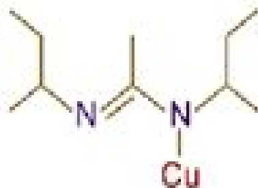
Cu(I)-N,N'-di-sec-butyl-acetamidinate (1)
