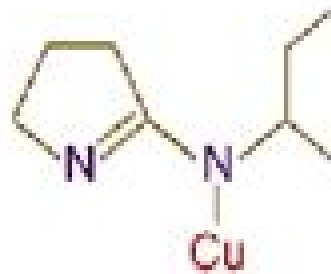
Cu(I)-N-sec-butyl-2-iminopyrrolidinate (3)
