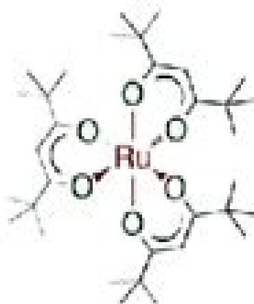
Ru(III)-tris(2,2,6,6-tetramethyl-3,5-heptanedionate) (4)
