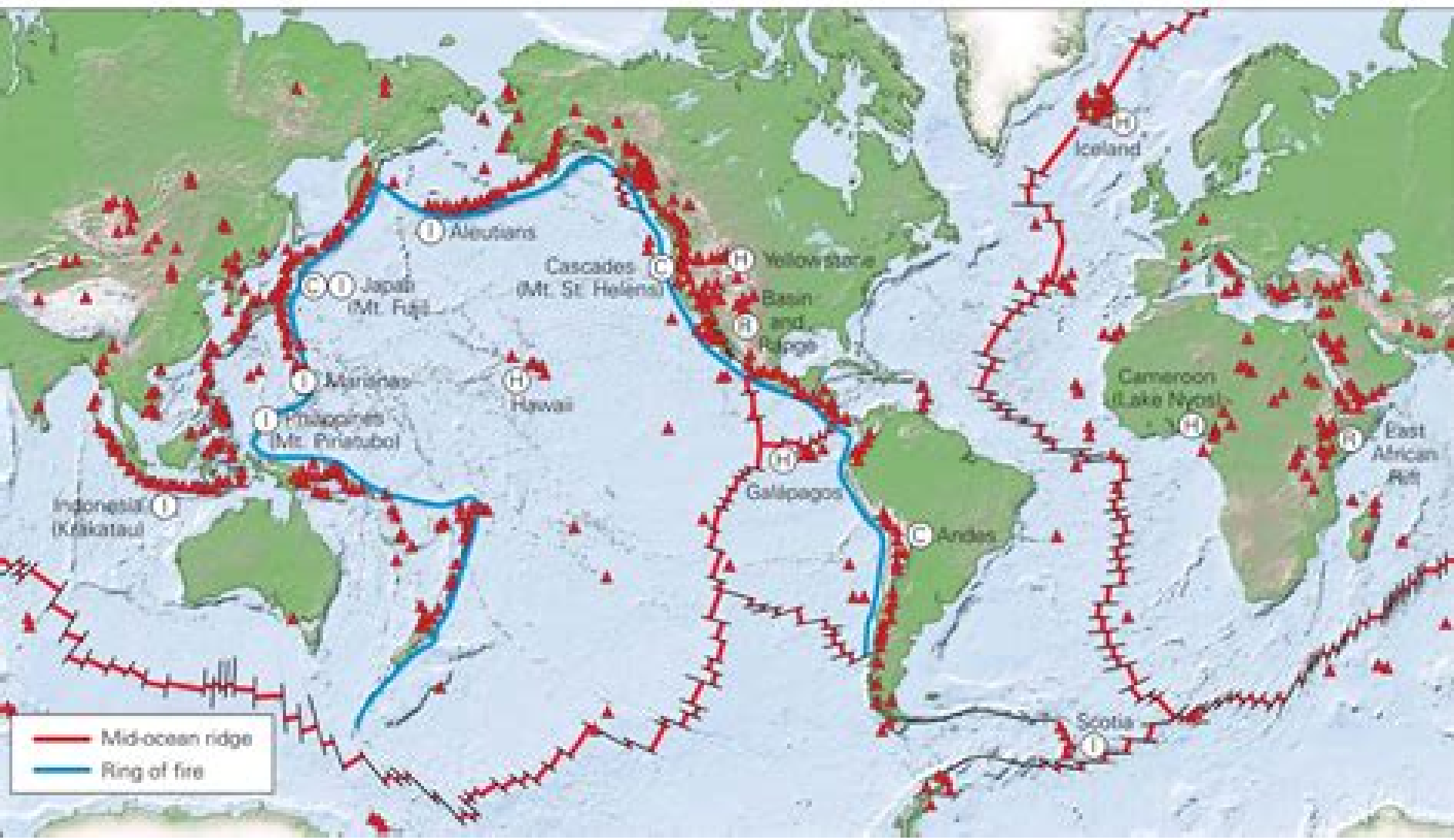
① = Island arc
