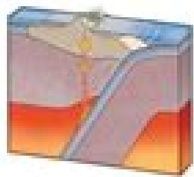
① = Island arc
