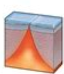
⑤ = Mid-ocean ridge
