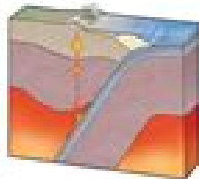
② = Continental arc
