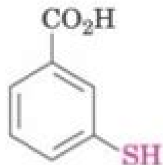
m -Mercaptobenzoic acid
