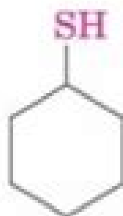
Cyclohexanethiol
