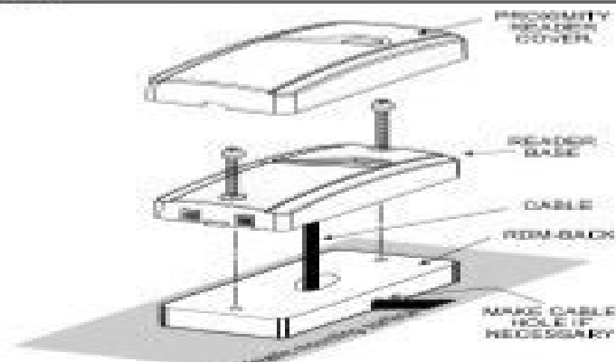
Figure 3. RDM-4 Mounting
