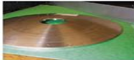
Plate. Bent orifice plates also can produce bias errors. This plate's inner edge, which should be flush with the tabletop, has become elevated, or bent, about 3/8 in. from flatness.
